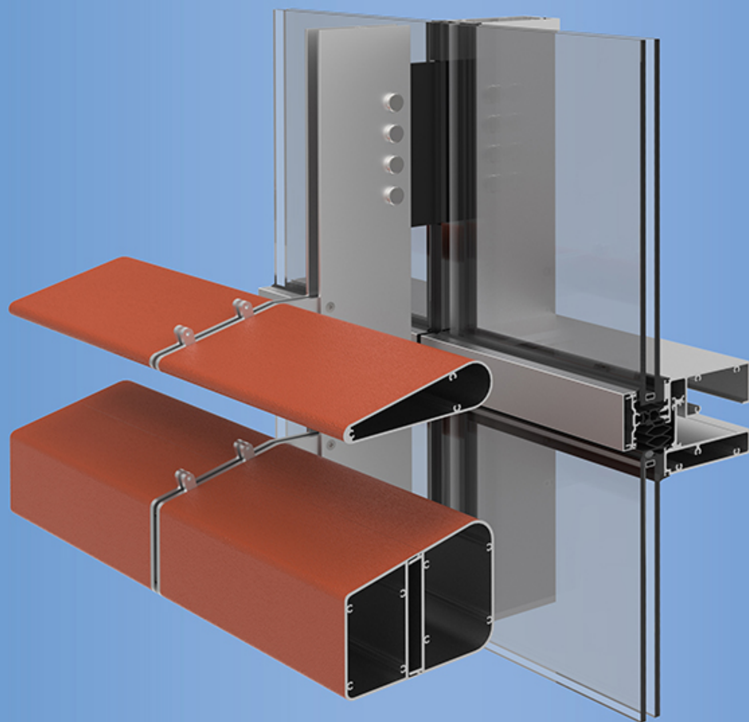
YUW 750 XT Unitized Curtain Wall with Sunshade
