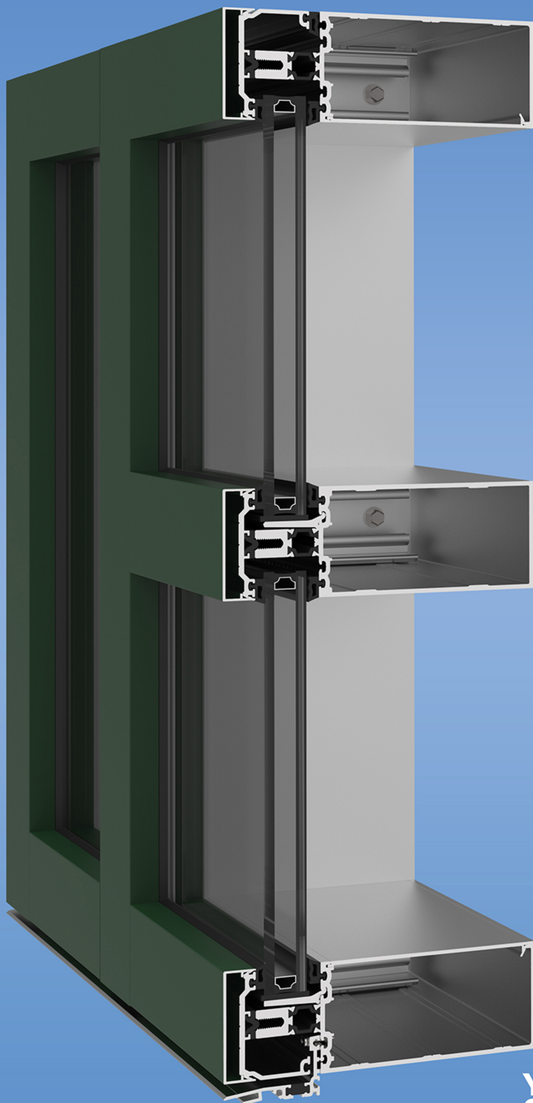
YCW 750 XT Curtain Wall System
